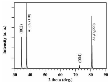
Fig. 2. X-ray diffraction pattern of ZnO nanowires on a sapphire substrate. Only (000 l ) peaks are observed, owing to their well-oriented growth configuration. The diffraction pattern is taken on a Siemens Z5000 x-ray diffractometer. a.u., arbitrary units.
