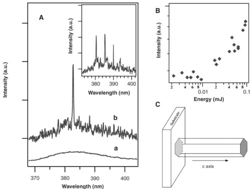
Fig. 3. (A) Emission spectra from nanowire arrays below (line a) and above (line b and inset) the lasing threshold. The pump power for these spectra are 20, 100, and 150 kW/cm 2 , respectively. The spectra are offset for easy comparison. (B) Integrated emission intensity from nanowires as a function of optical pumping energy intensity. (C) Schematic illustration of a nanowire as a resonance cavity with two naturally faceted hexagonal end faces acting as reflecting mirrors. Stimulated emission from the nanowires was collected in the direction along the nanowire's end-plane normal (the symmetric axis) with a monochromator (ISA, Edison, New Jersey) combined with a Peltier-cooled charge-coupled device (EG&G, Gaithersburg, Maryland). The 266-nm pump beam was focused to the nanowire array at an angle 10° to the end-plane normal. All experiments were carried out at room temperature.
