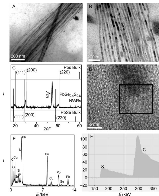
Figure 1. Structural characterization of \text{PbSe}_{0.4}\text{S}_{0.6} core-shell nanowires. A) \text{PbSe} nanowires before \text{PbS} addition, B) the resulting \text{PbSe}_{0.4}\text{S}_{0.6} alloy nanowires, C) powder XRD pattern of \text{PbSeS} alloy nanowires, D) HRTEM image of a single nanowire, E) EDX spectrum taken from the selected area denoted by a black square shown in (D), and F) an EELS spectrum of the same area.
