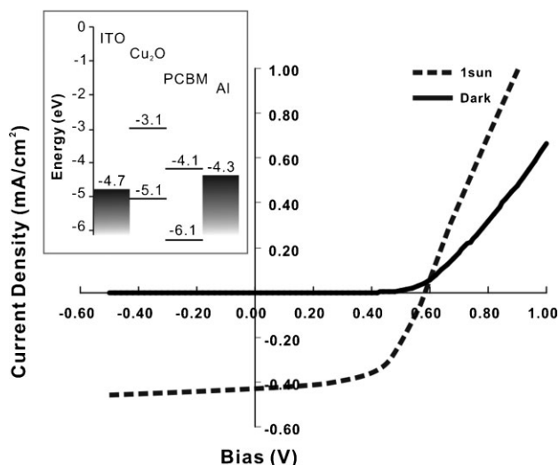
Figure 4. I - V characteristics of the ITO/Cu 2 O (200 nm)/PCBM/Al device in dark and under AM 1.5 and 1 Sun illumination. The inset shows the energy diagram of the device.
