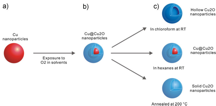
Scheme 1. Oxidation of the Cu NPs to generate different monodisperse nanostructures.
