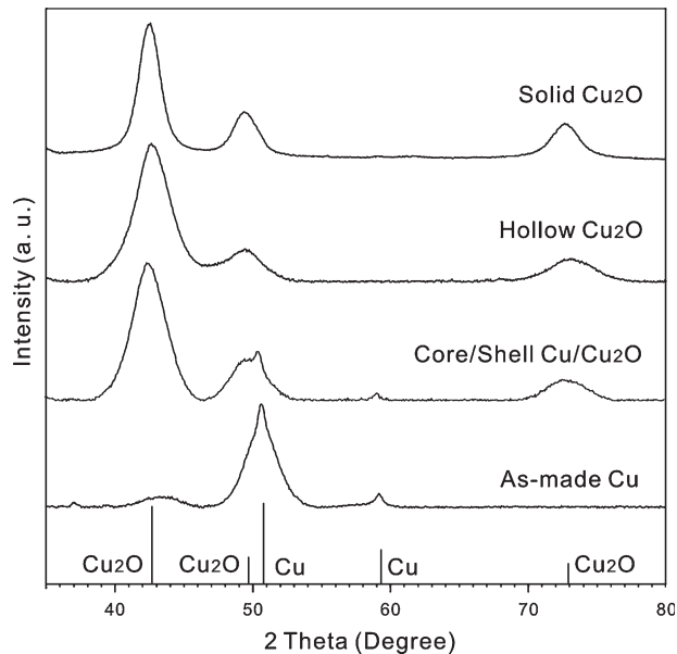
Figure 2. Powder XRD patterns of the as-synthesized Cu, Cu@Cu 2 O, hollow Cu 2 O, and solid Cu 2 O NPs.
