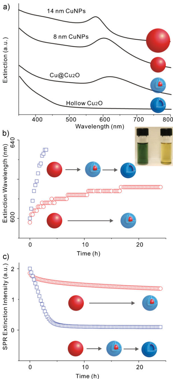
Figure 3. a) Absorbance spectra of Cu NPs of different sizes and structures. b) SPR wavelengths and c) intensities plotted as functions of time for NPs dispersed in hexane and chloroform. The inset shows the color of NPs dispersed in chloroform (yellow) and hexane (green) after UV-vis measurement.
