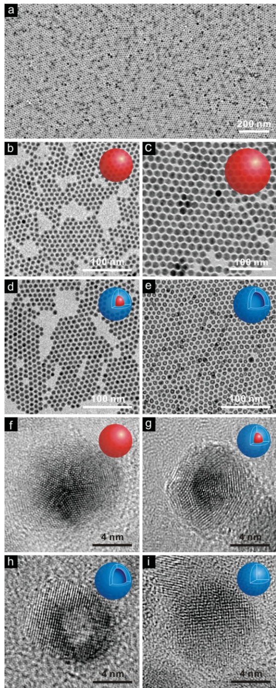
Figure 1. TEM images of: a) a large-area view of the self-assembled Cu NPs, b) the 8-nm Cu NPs, c) the 14-nm Cu NPs, d) the Cu@Cu 2 O NPs, and e) the hollow Cu 2 O NPs. HRTEM images of: the f) Cu, g) Cu@Cu 2 O, h) hollow Cu 2 O, and i) solid Cu 2 O NPs.
